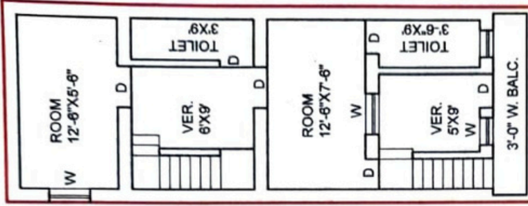
4TH FLOOR PLAN
